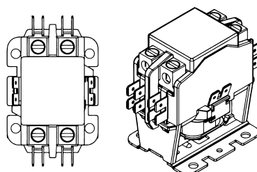
Contactor 2 Polos
